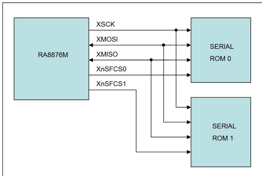
圖 16-3 : RA8876M Serial Flash/ROM System
