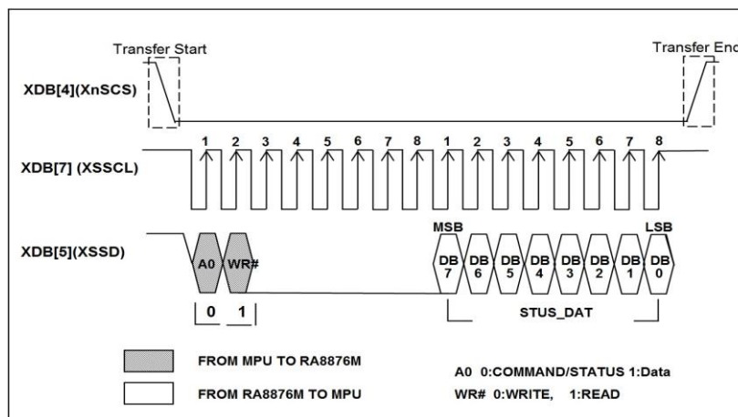
圖 7-8 : Status Read on 3-Wire SPI-Bus
