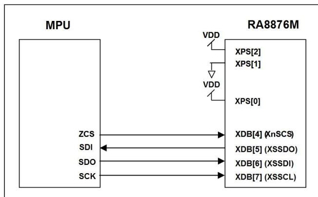
圖 7-13 : The MPU Interface Diagram of 4-Wire SPI
