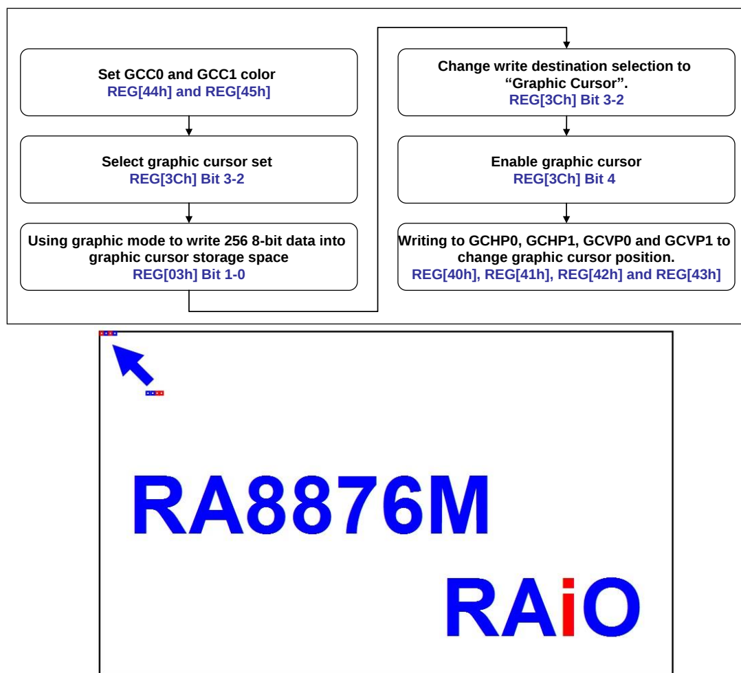
圖 14-21 : The Display with Graphic Cursor
